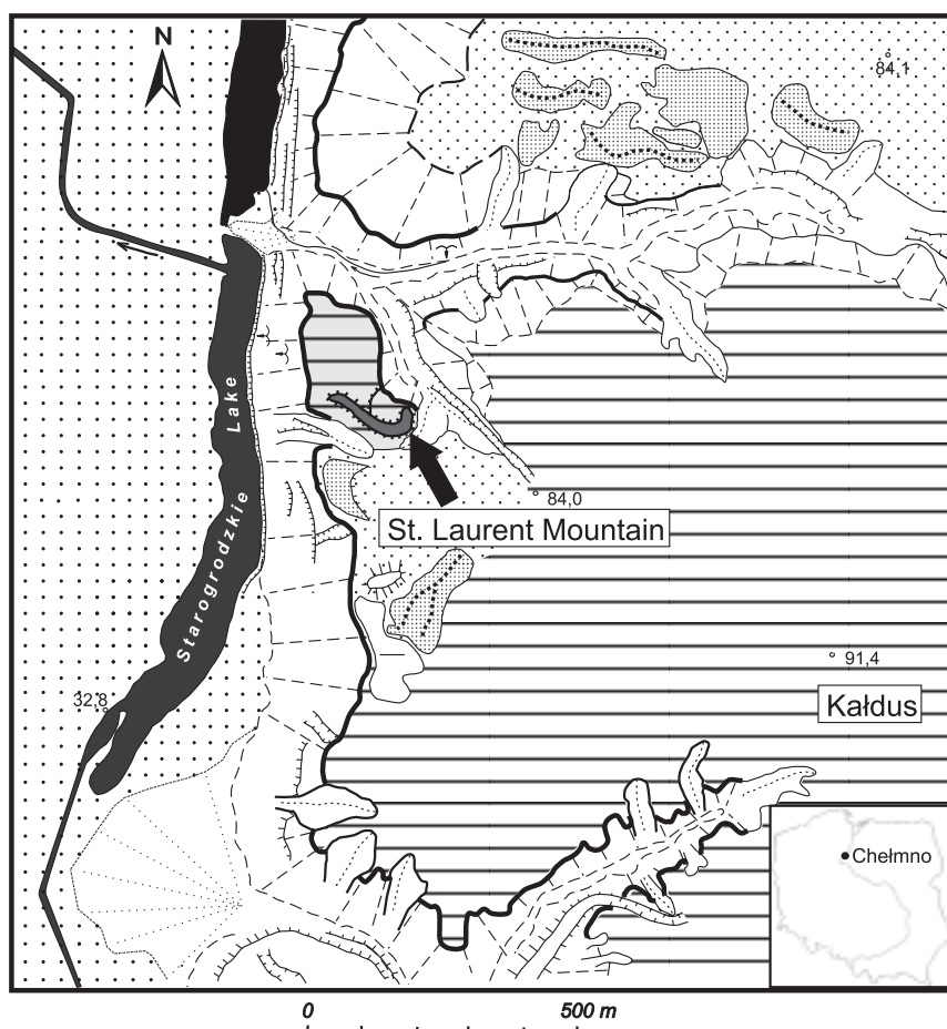
Fig 1. Geomorphological and hydrological sketch of the researched area in Kaldus.
