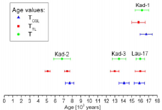
Fig. 5. Luminescence dating results. The mean age T was calculated from averaging ED_{OSL} and ED_{TL} values. For comparison the T_{OSL} and T_{TL} dates are also shown.
